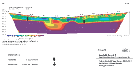
Geolectrical section 4, the 'dromos' in the bedrock is clearly visible (graphics: GGH).
